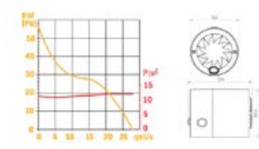
Air Flow - Static Pressure Characteristics
