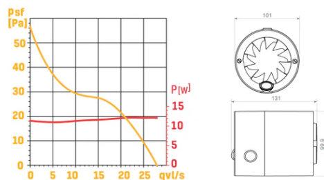
Air Flow - Static Pressure Characteristics
